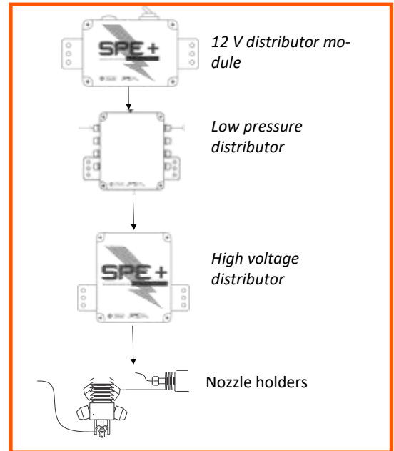
SPE kit for boom sprayer
